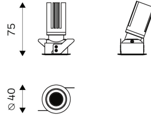
CUT-OUT: \varnothing 35mm
