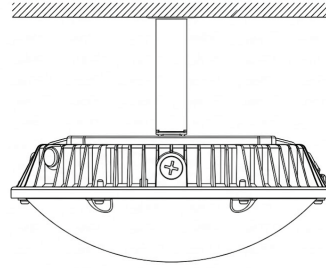
Pole Mount
